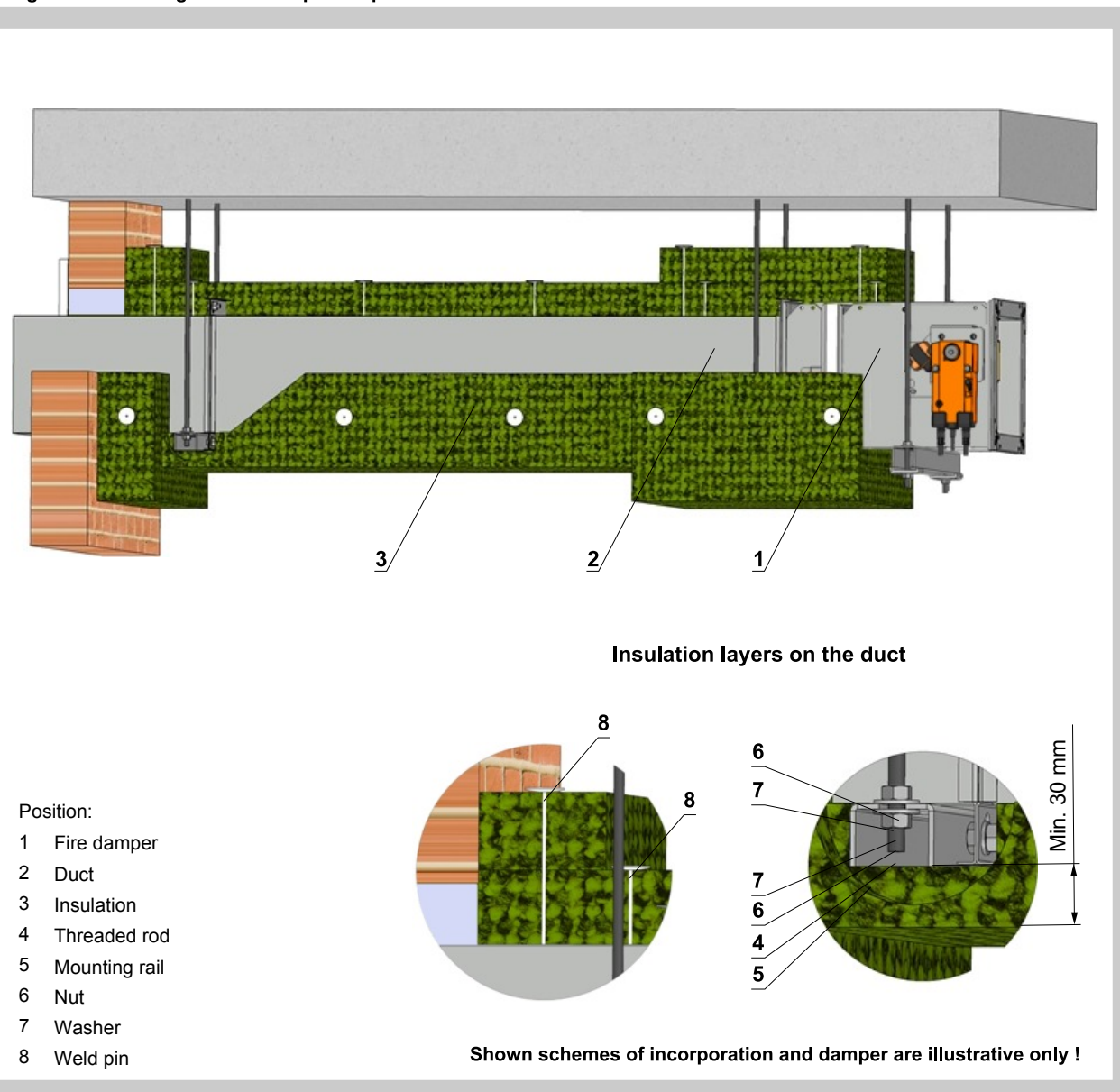
Fig. 83 Rectangular fire damper suspension on the wall - horizontal installation
