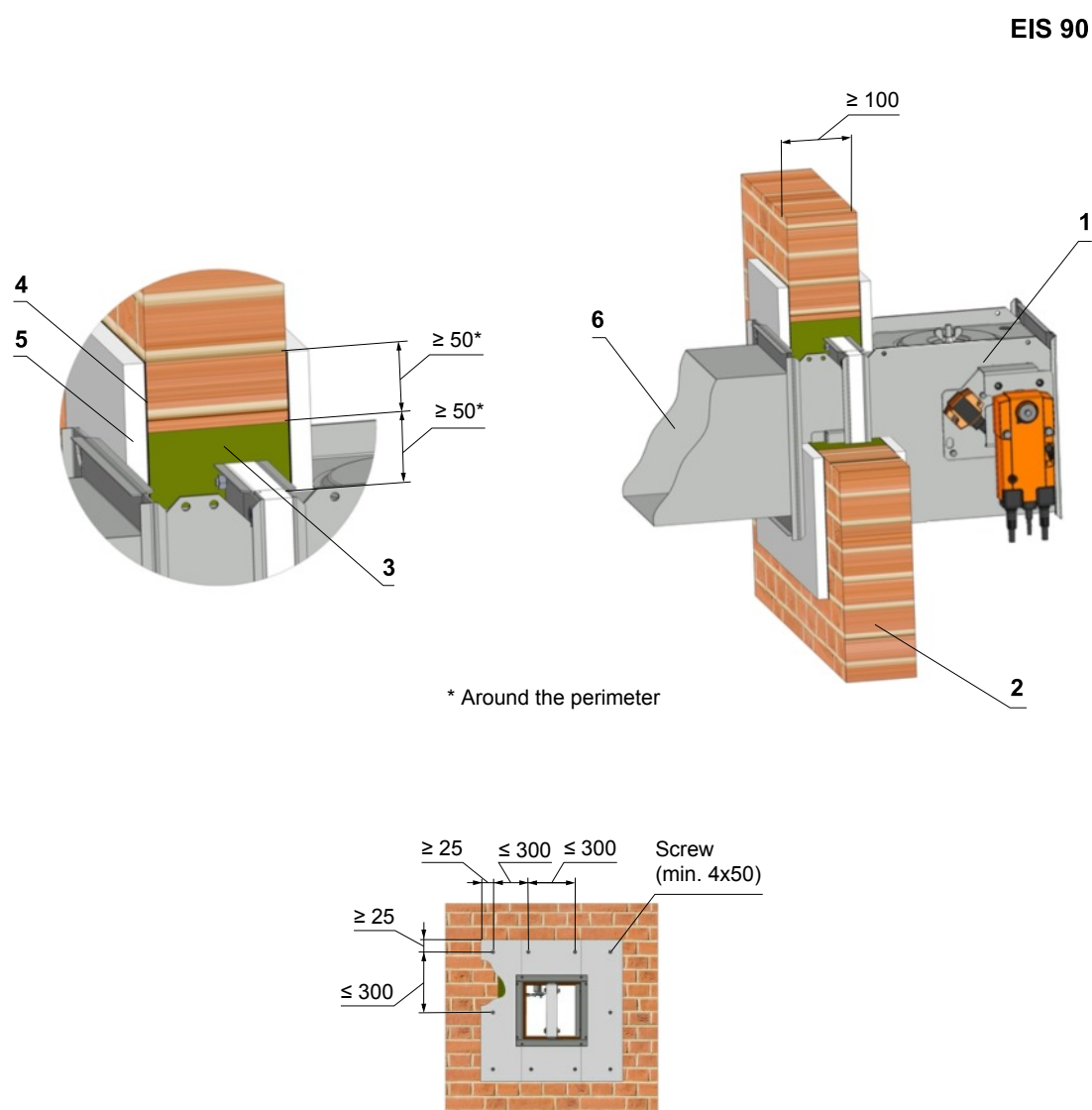
Fig. 38 Solid wall construction - stuffing box, fire protection mastic and cement lime plate
