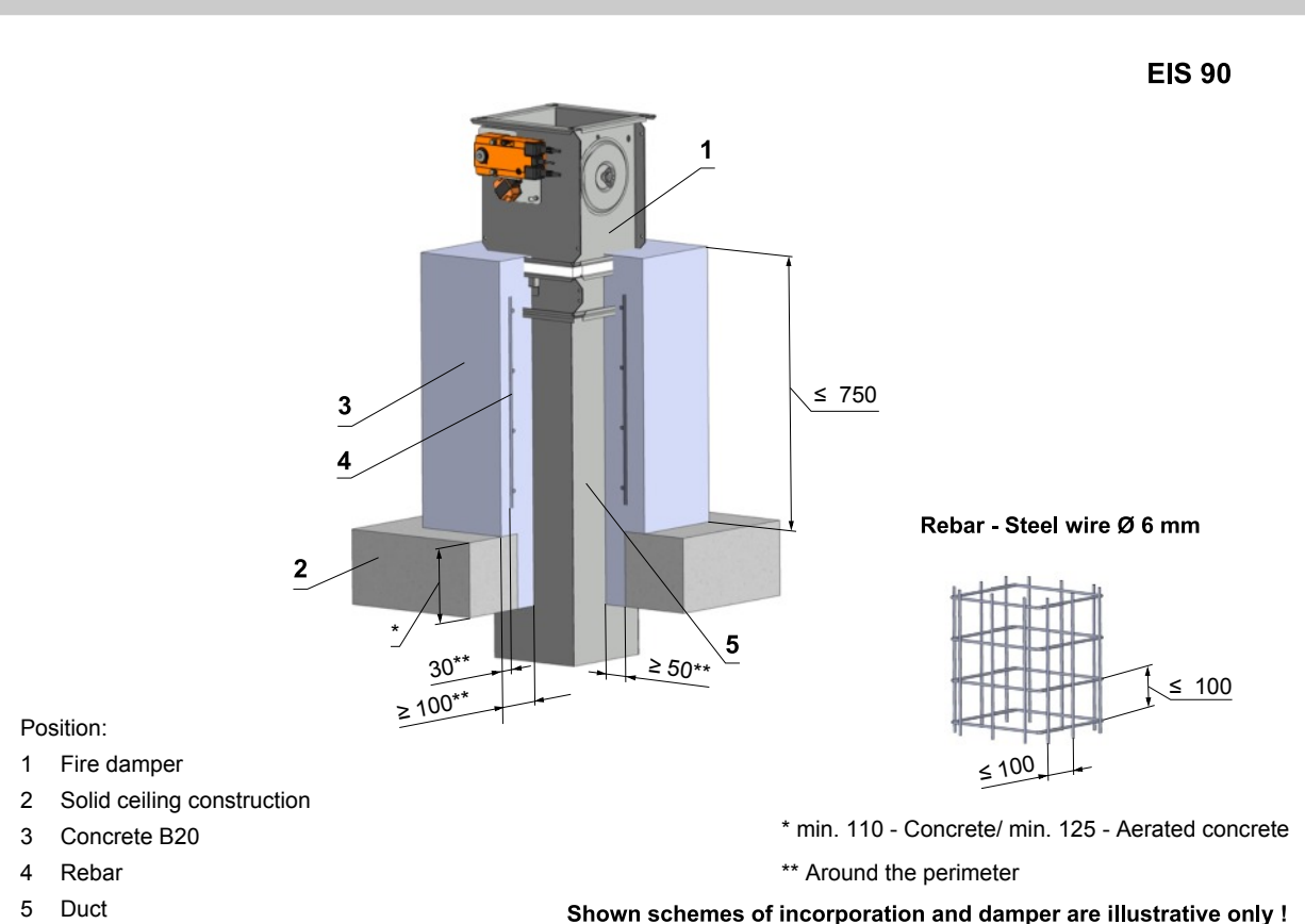
Fig. 65 Outside solid ceiling construction - concrete
