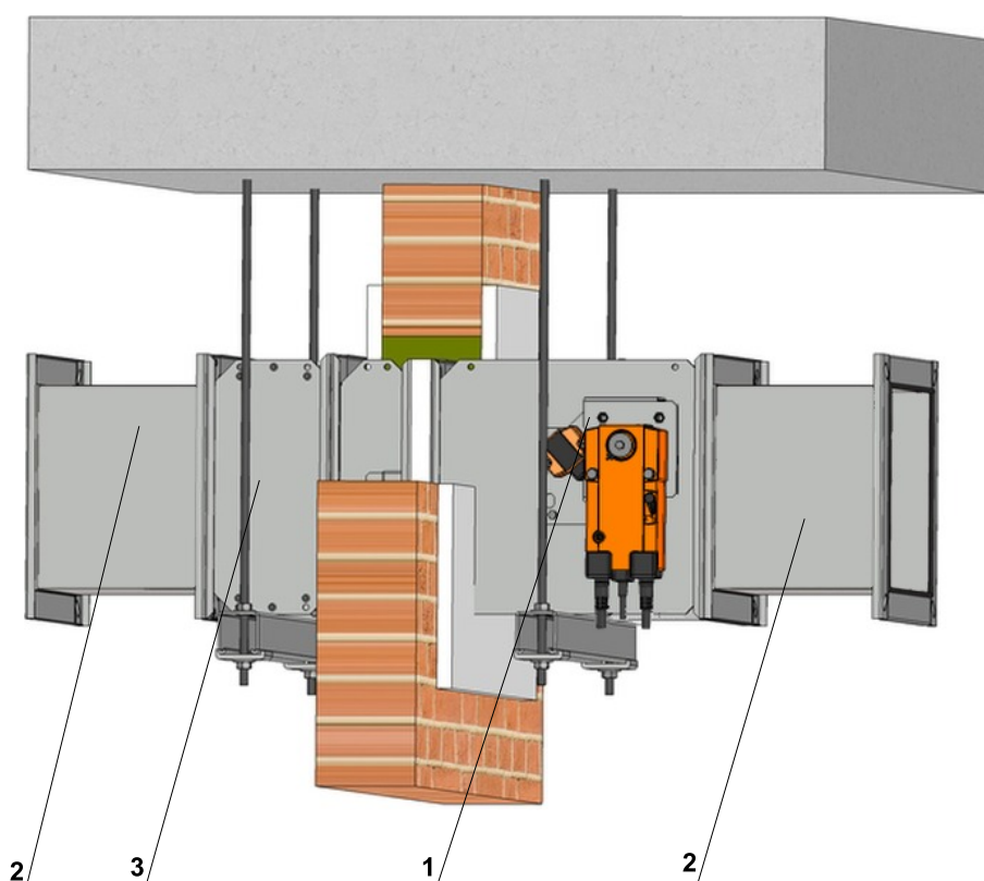
Fig. 81 Suspension - horizontal duct
