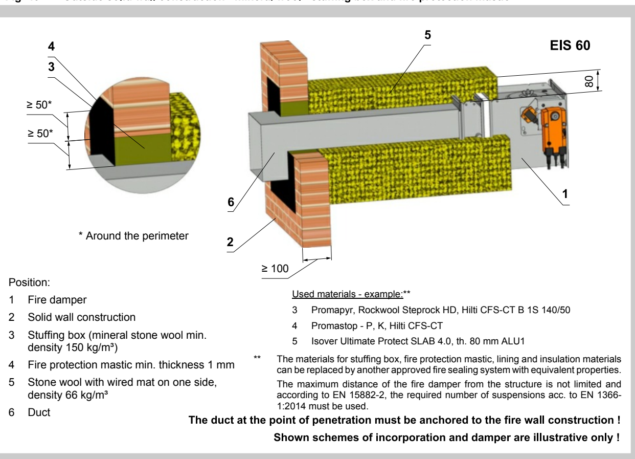
Fig. 43 Outside solid wall construction - mineral wool - stuffing box and fire protection mastic
