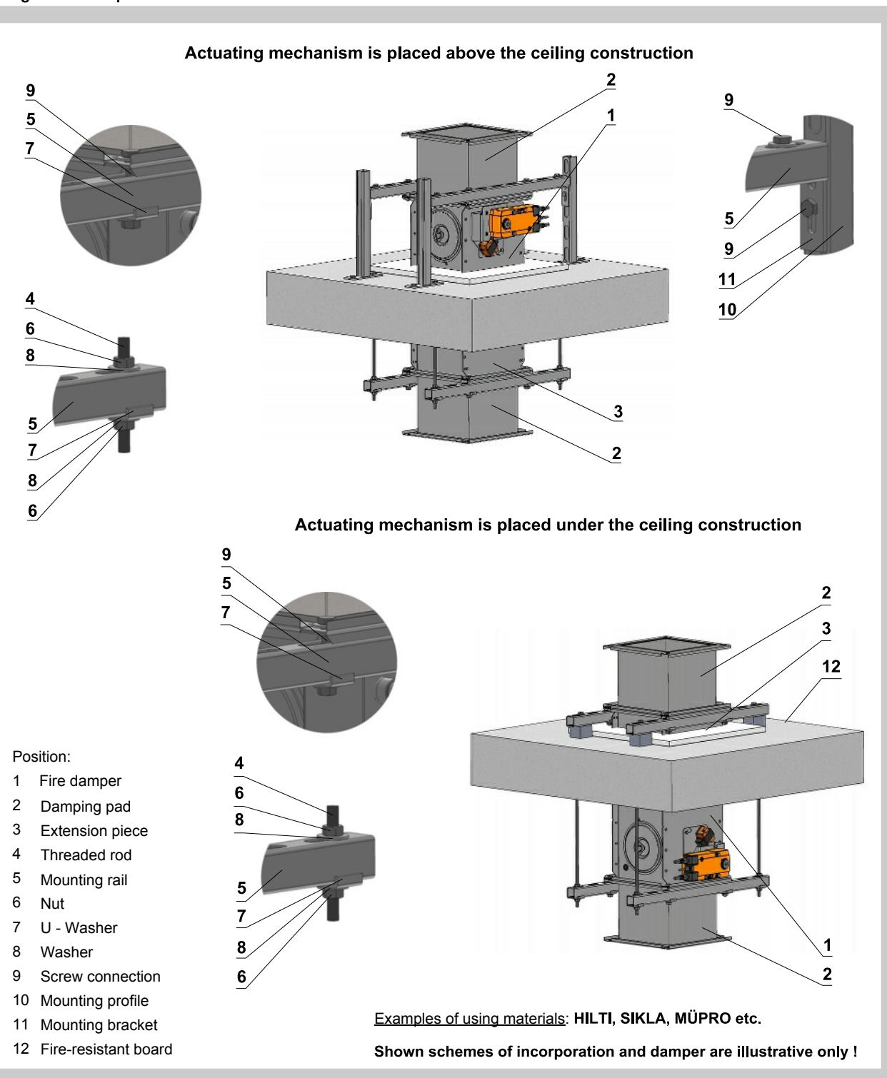
Fig. 82 Suspension - vertical duct
