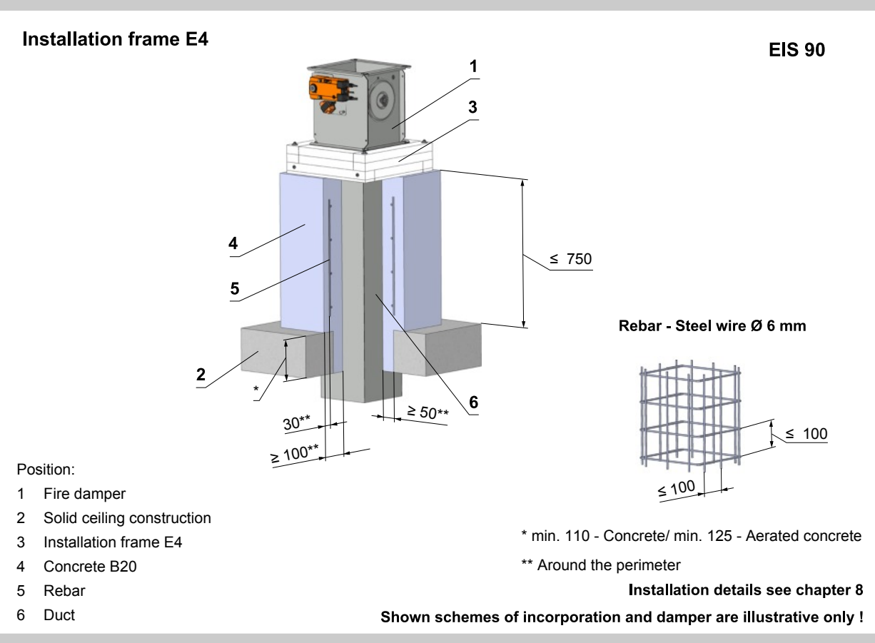
Fig. 66 Outside solid ceiling construction - concrete - installation frame E4
