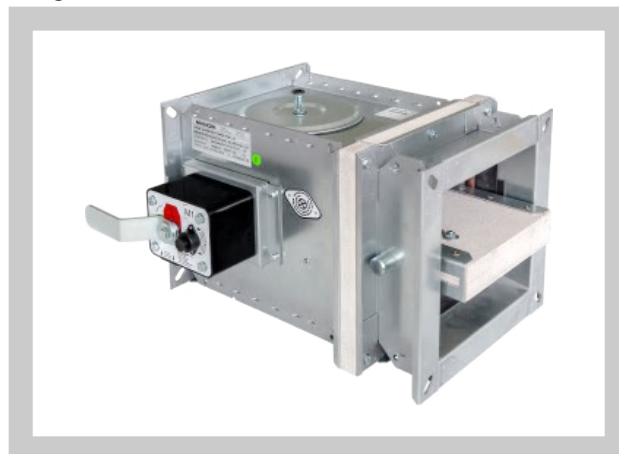
Fig. 2 FDMQ with mechanical control
