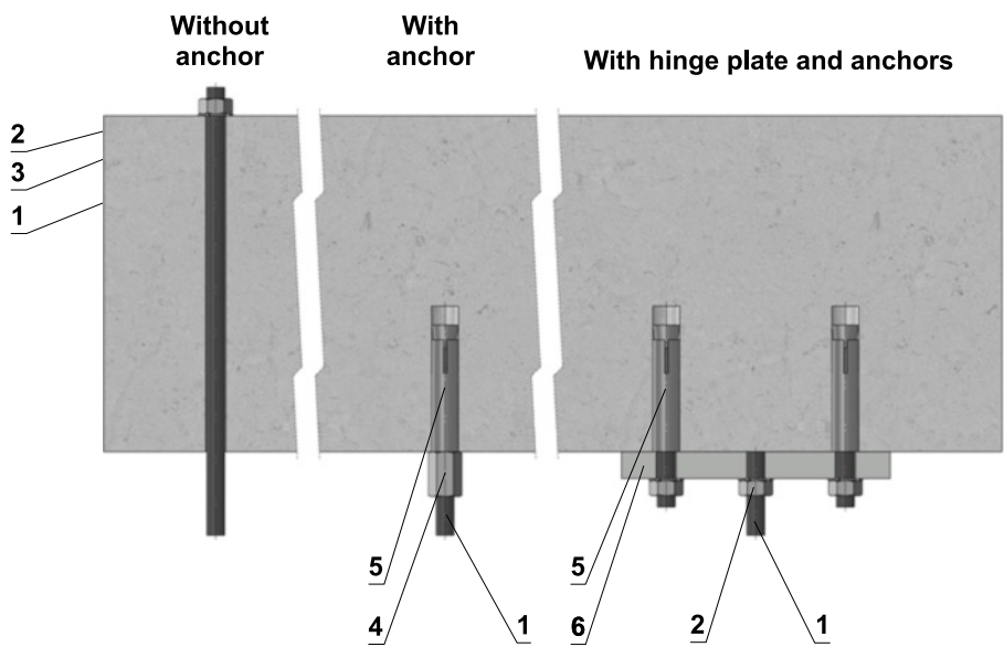
Hinge plates
