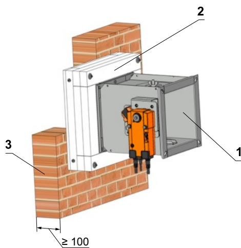
Installation frame E4
