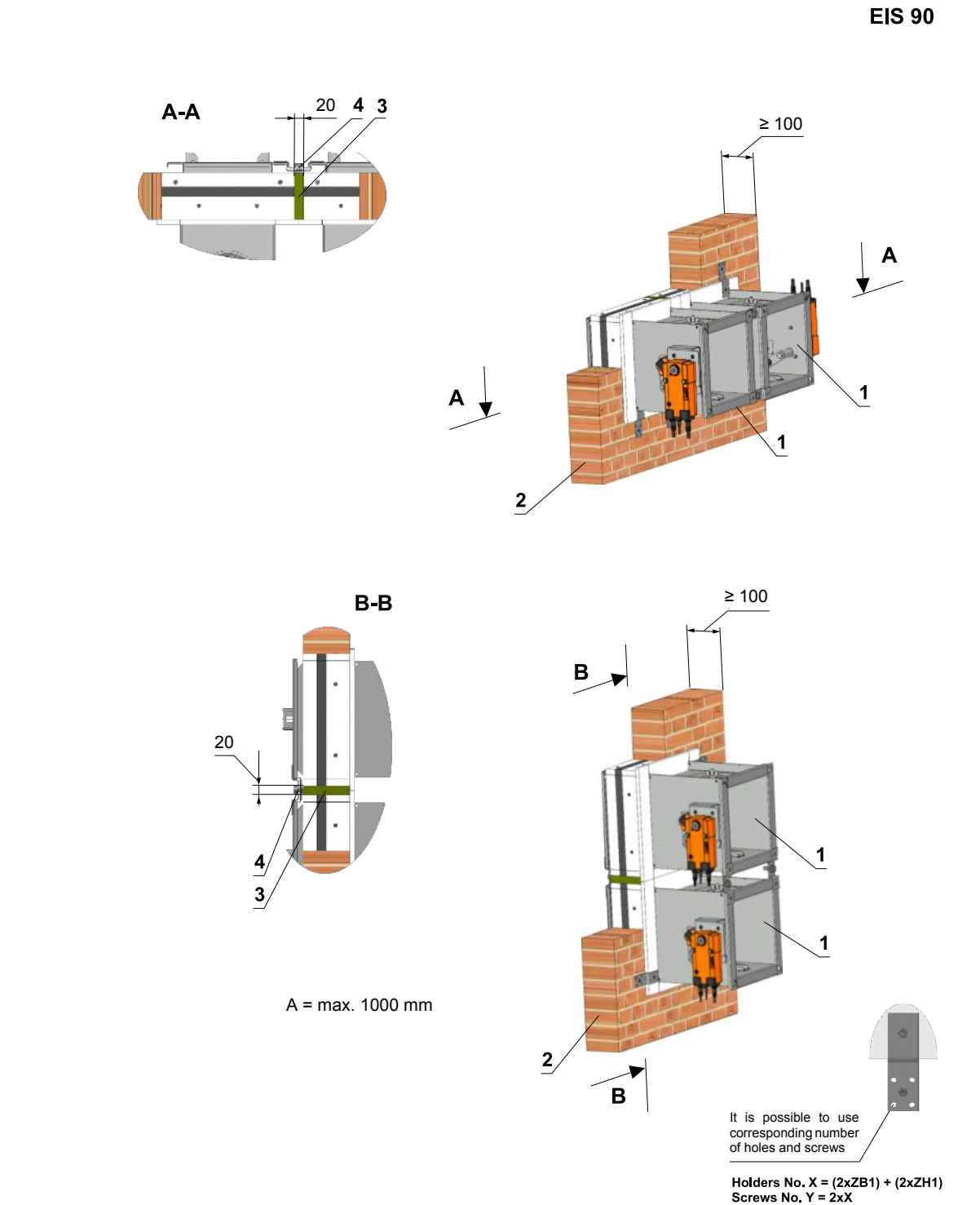
Fig. 41 Solid wall construction - battery - installation frame E1
