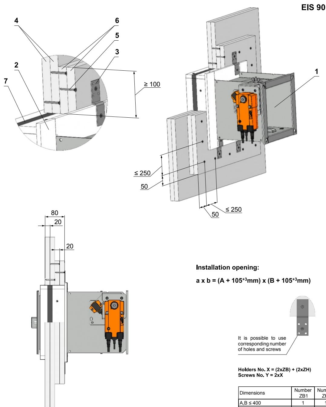
Fig. 70 Thin shaft wall - installation frame E1
