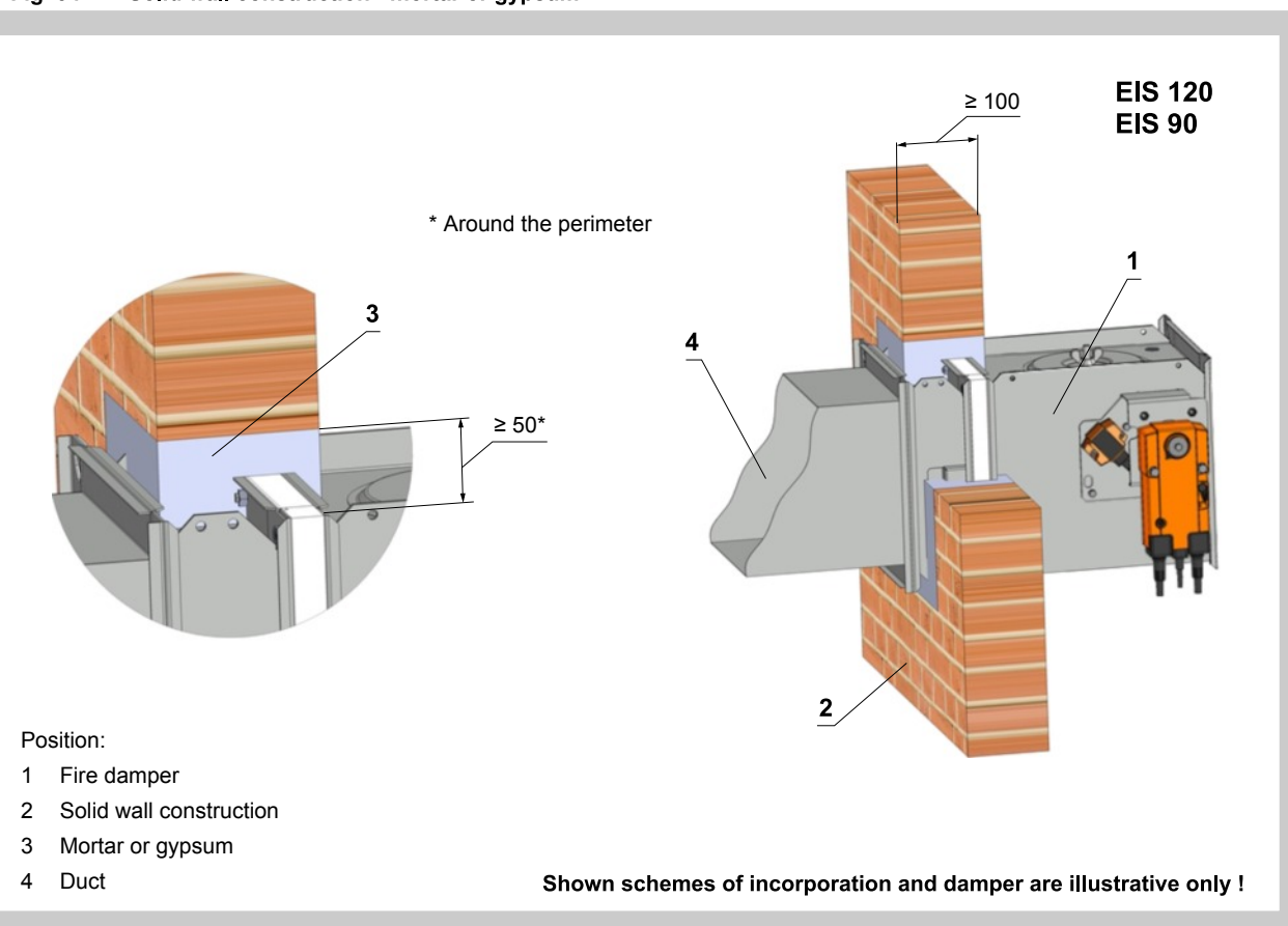
Fig. 34 Solid wall construction - mortar or gypsum
