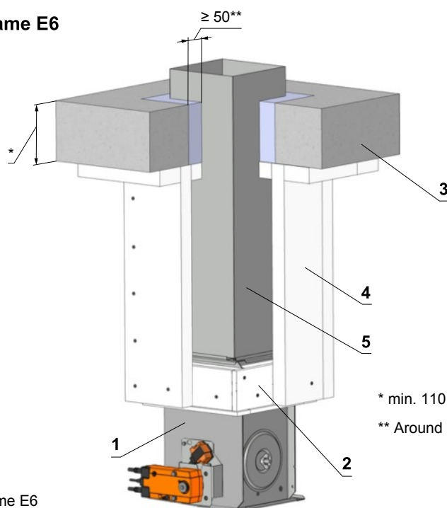
Fig. 67 Outside solid ceiling construction - installation frame E6 with cement lime plates
