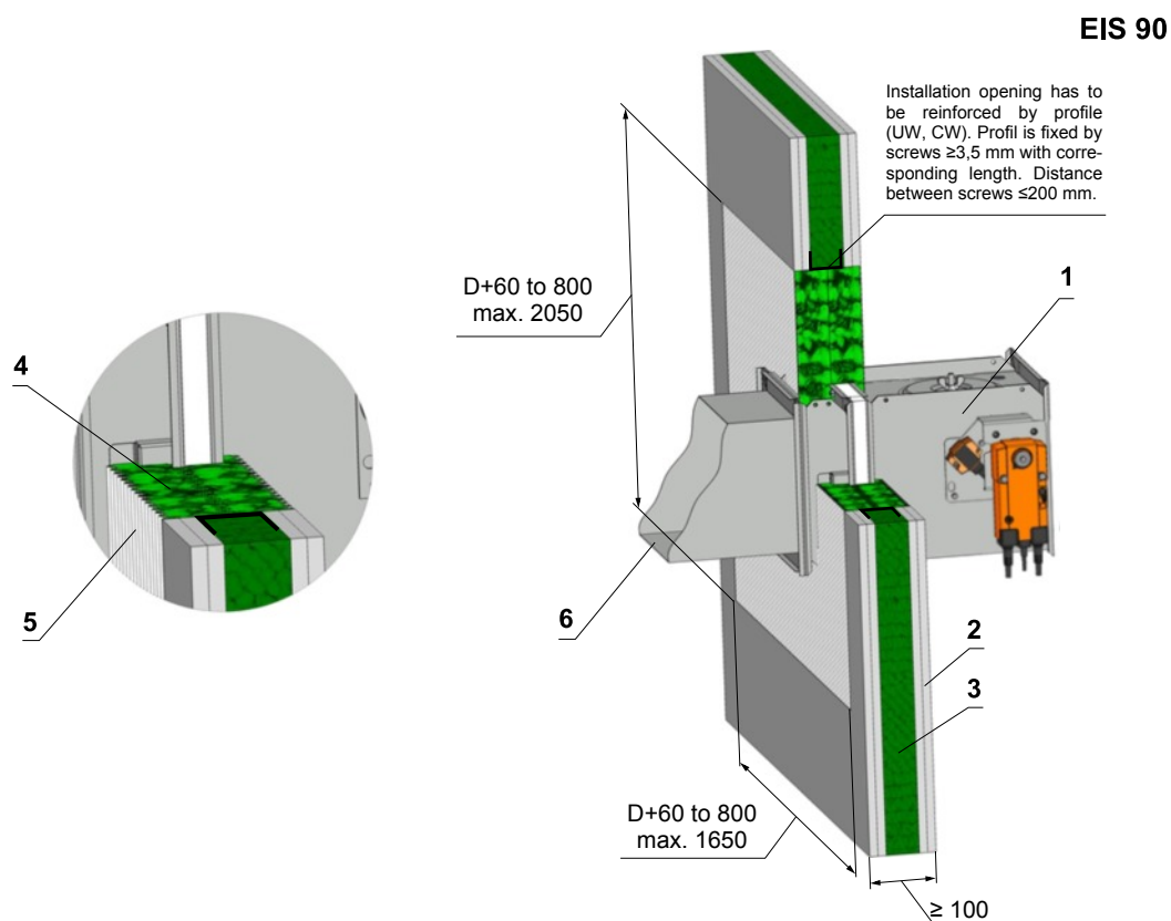
Fig. 52 Gypsum wall construction - Weichschott
