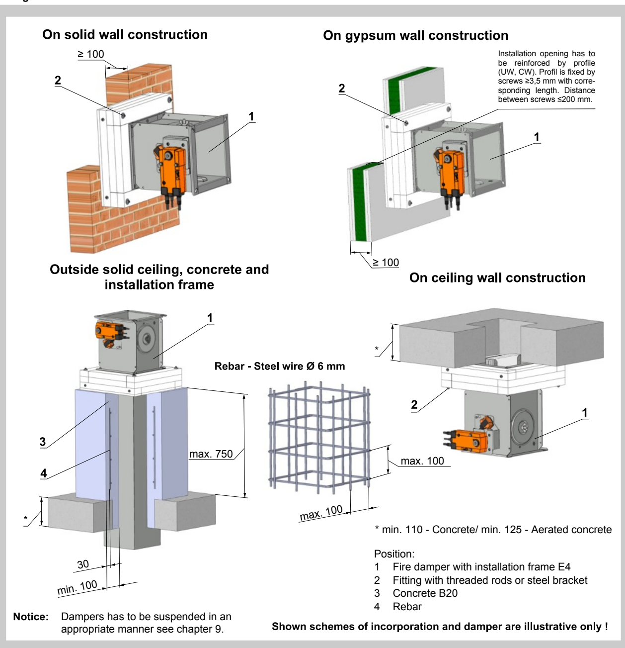
Fig. 75 Installation frame E4
