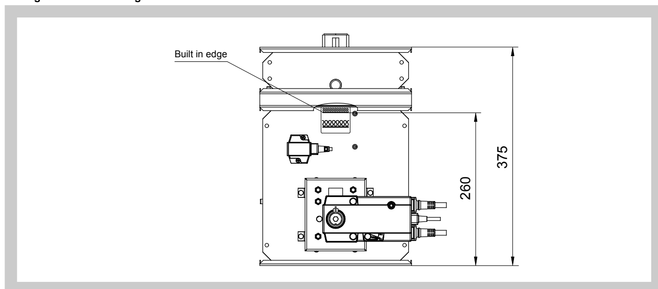
Fig. 32 Built in edge
