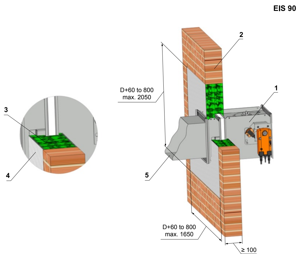
Fig. 40 Solid wall construction - Weichschott
