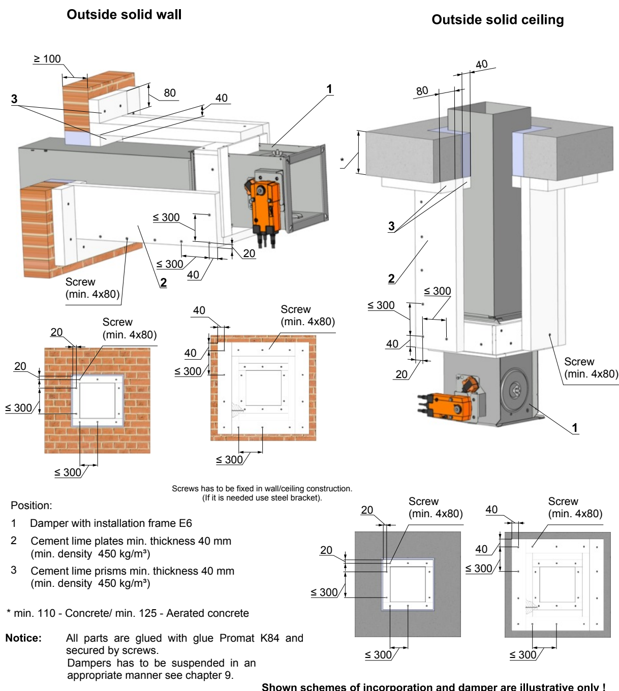
Fig. 77 Installation frame E6
