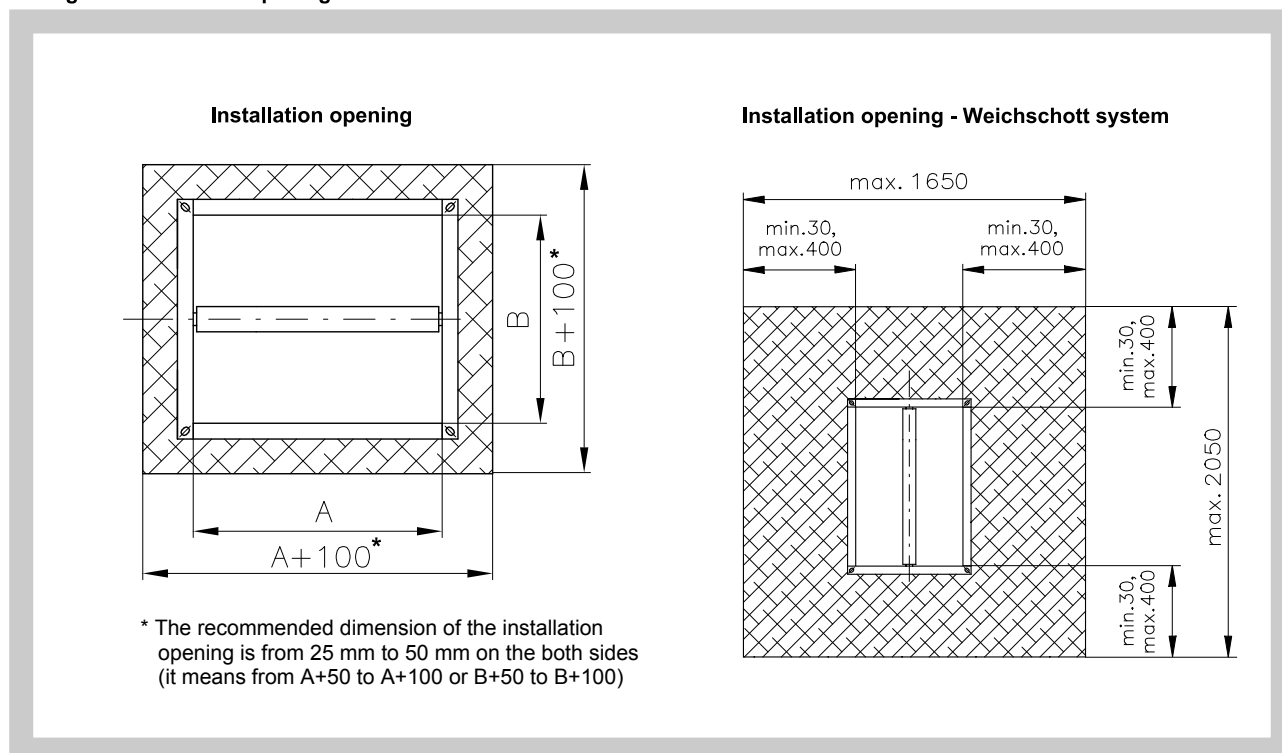
Fig. 33 Installation opening dimensions
