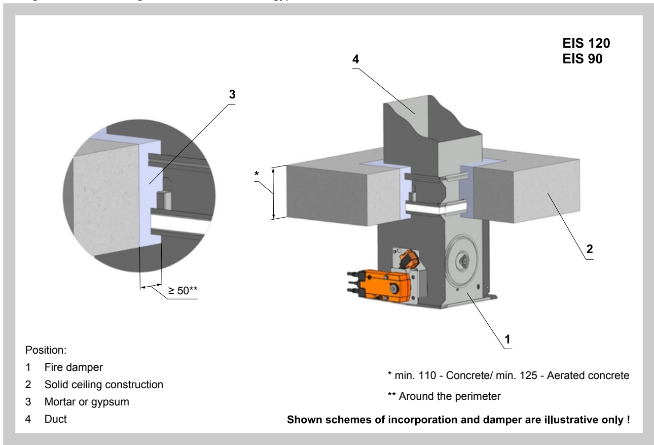
Fig. 58 Solid ceiling construction - mortar or gypsum
