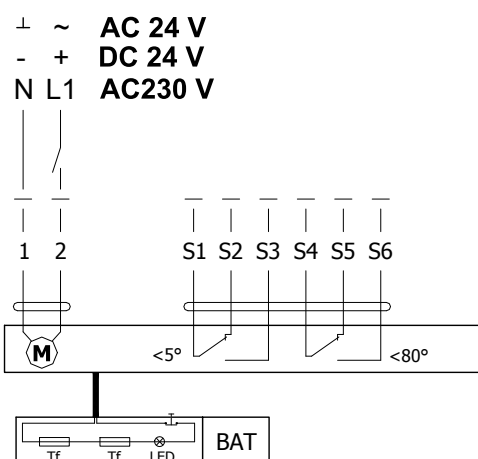
Fig. 11 Actuating mechanism BELIMO BF 230-TN, BF 24-TN (-ST)
