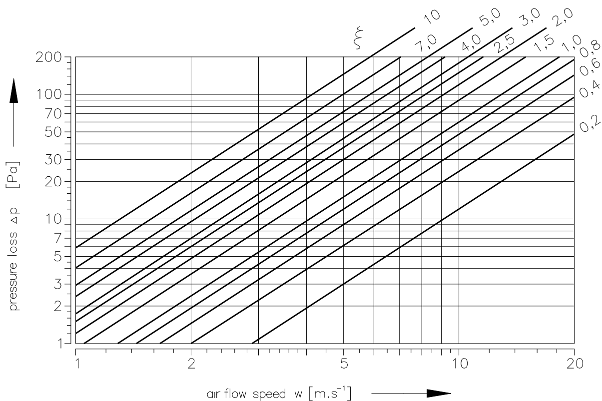
Diagram 10.2.1. Pressure losses for air density \rho = 1,2 \text{ kg.m}^3
