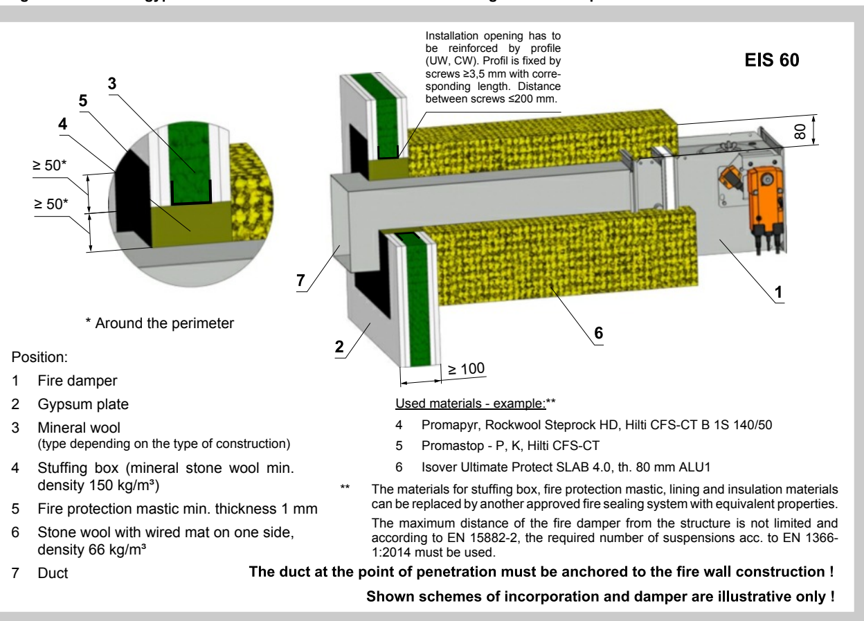
Fig. 56 Outside gypsum wall construction - mineral wool - stuffing box and fire protection mastic
