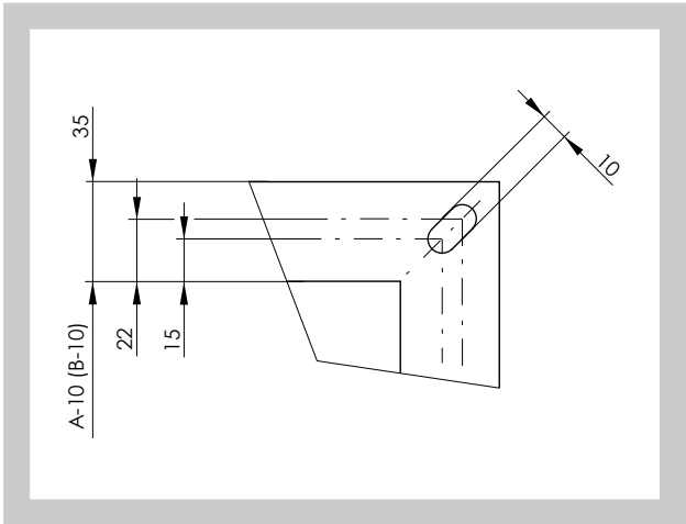
Fig. 30 Flange of Damper - INSTALLATIONS SIDE
