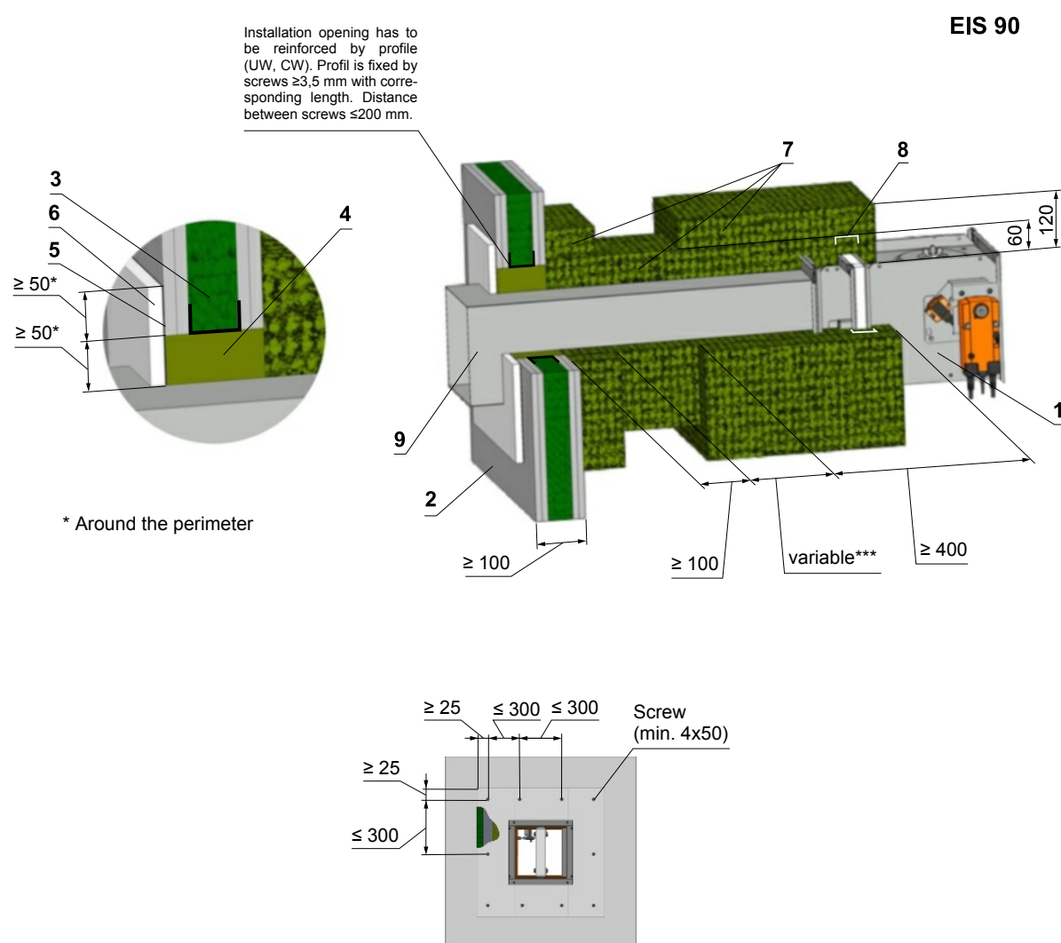
Fig. 57 Outside gypsum wall construction - mineral wool, stuffing box, fire protection mastic and cement lime plate
