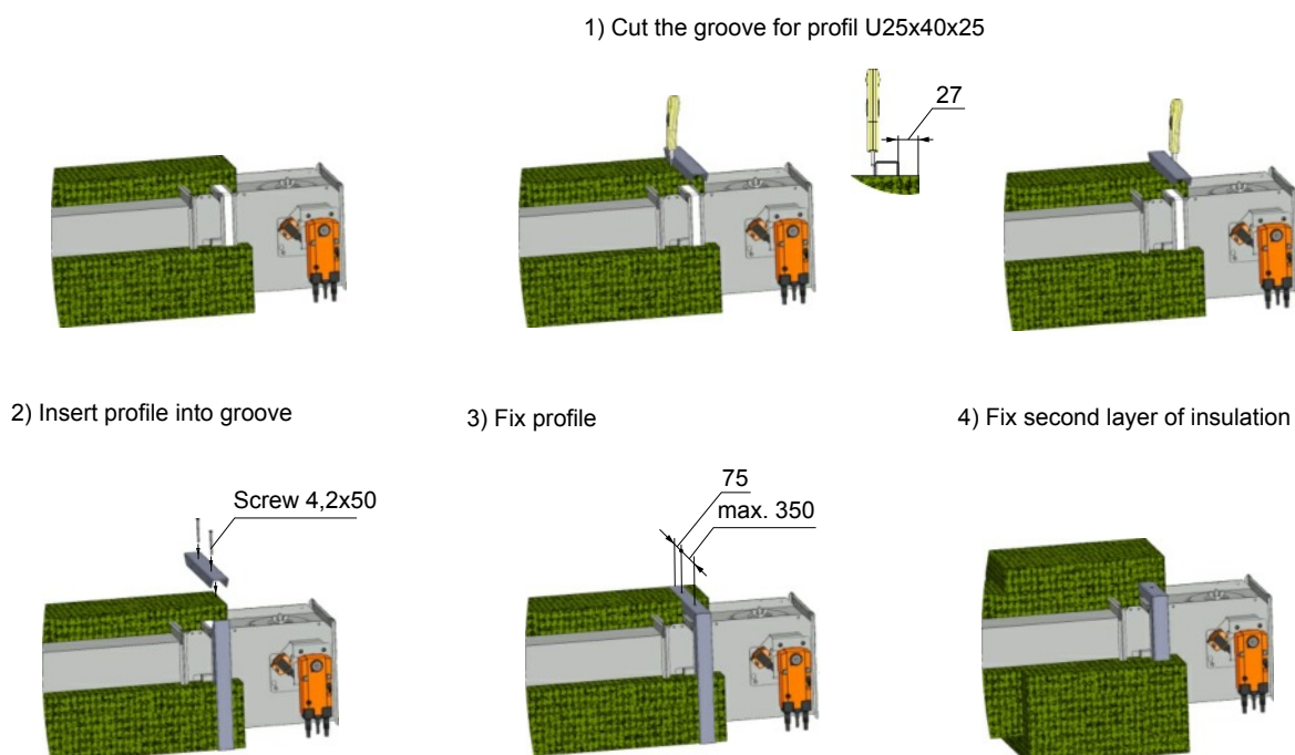
Fig. 79 Installation procedure
