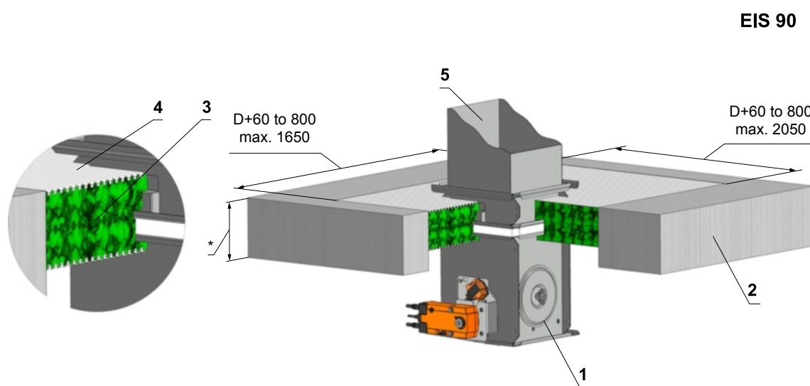
Fig. 62 Solid ceiling construction - Weichschott
