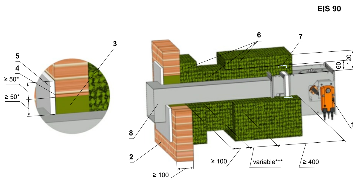
Fig. 44 Outside solid wall construction - mineral wool, stuffing box, fire protection mastic and cement lime plate
