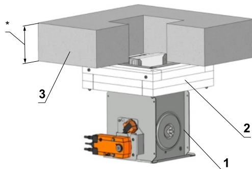
Installation frame E4
