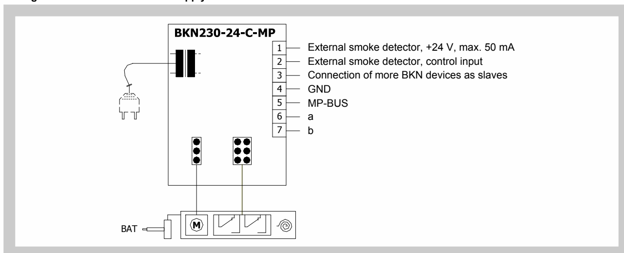
Fig. 17 Communication and supply device BKN 230-24-C-MP
